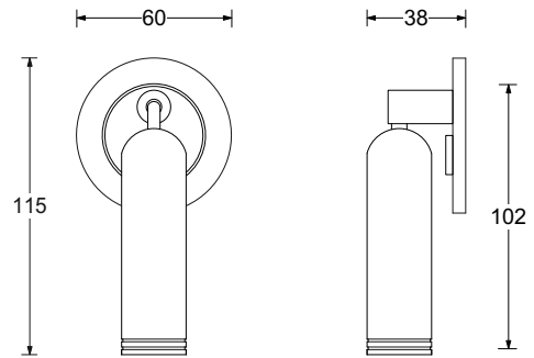
Dimensions in mm and approximate
