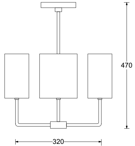
Dimensions in mm and approximate
