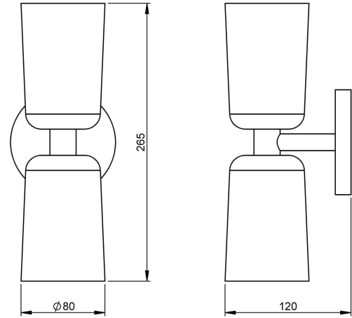
Dimensions in mm and approximate
